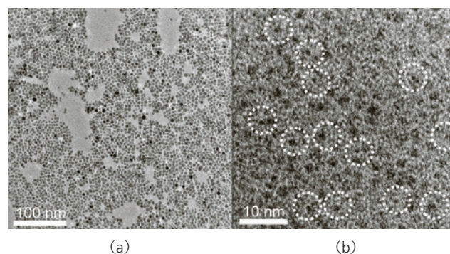
Figure 3 TEM images of (a) \text{Au}@ MSA nanoparticles and (b) \text{Au}_{25} . The clusters in (b) are seen only faintly since the size is \sim 1 nm. Some of the individual clusters are shown by circles. There are also cluster aggregates which upon extended electron beam irradiation fuse to form bigger particles
